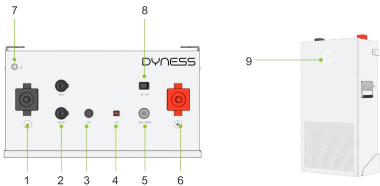
Figure 2-1 PowerBrick MAX the Sketch of Front Interface
