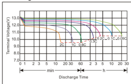
Discharge Current 25°C
